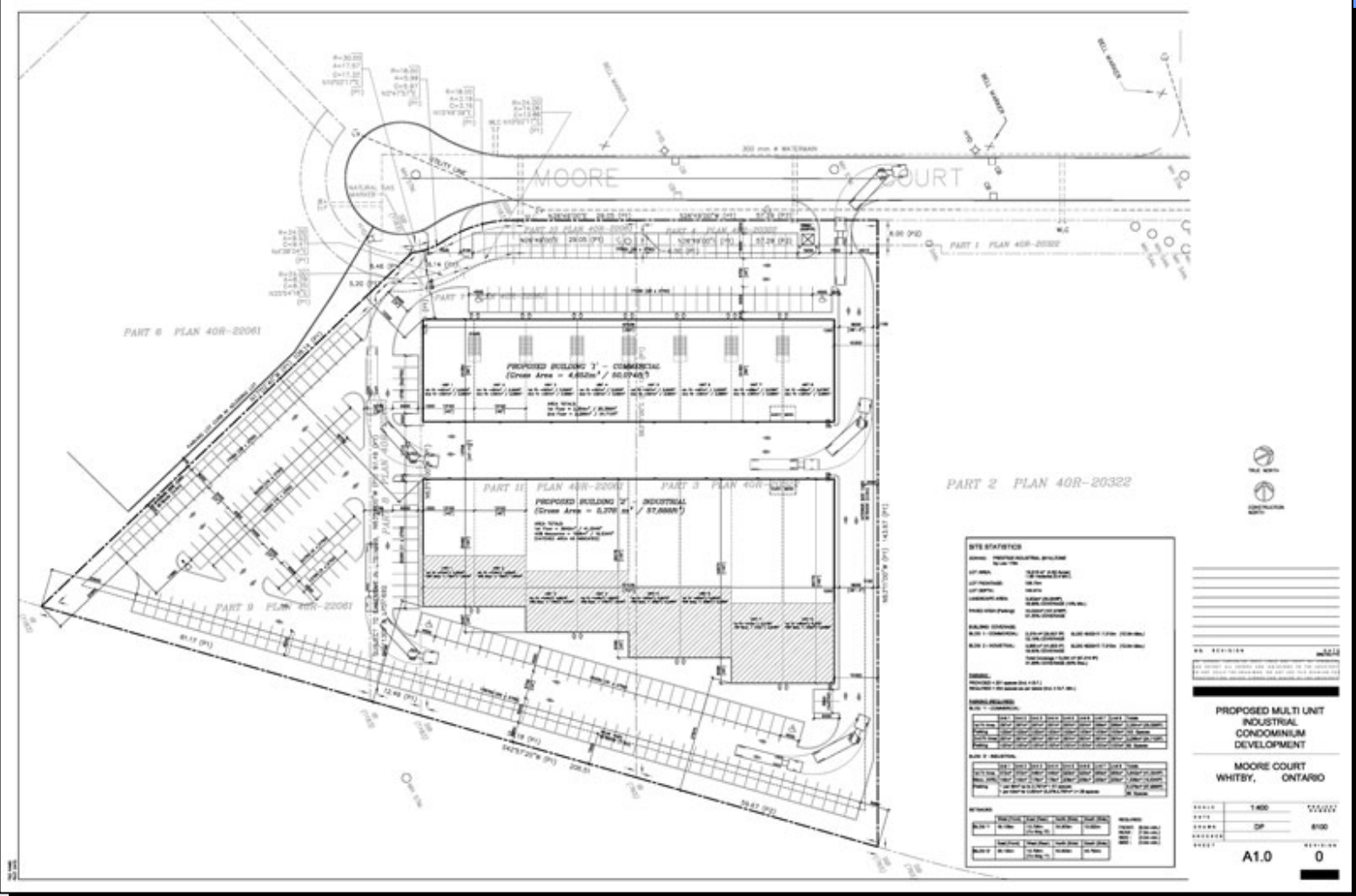
Site Plan Option 2: one industrial and one commercial building (click this link to enlarge)
