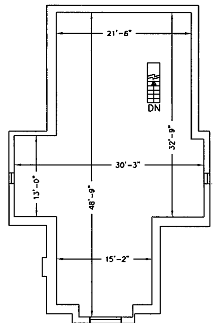
ATTIC GROSS AREA 1,247 SQ. FT.
