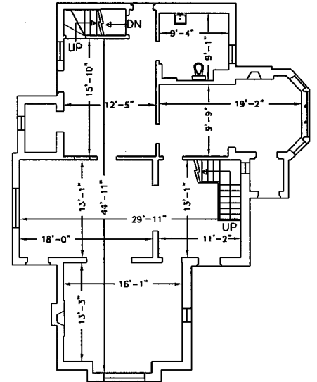
FIRST FLOOR GROSS AREA 1,428 SQ. FT.
