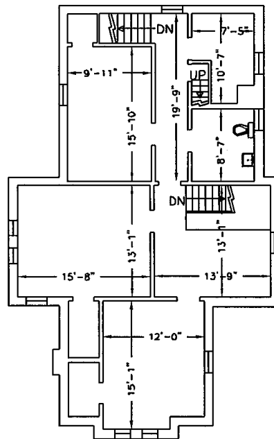
SECOND FLOOR GROSS AREA 1,247 SQ. FT.
